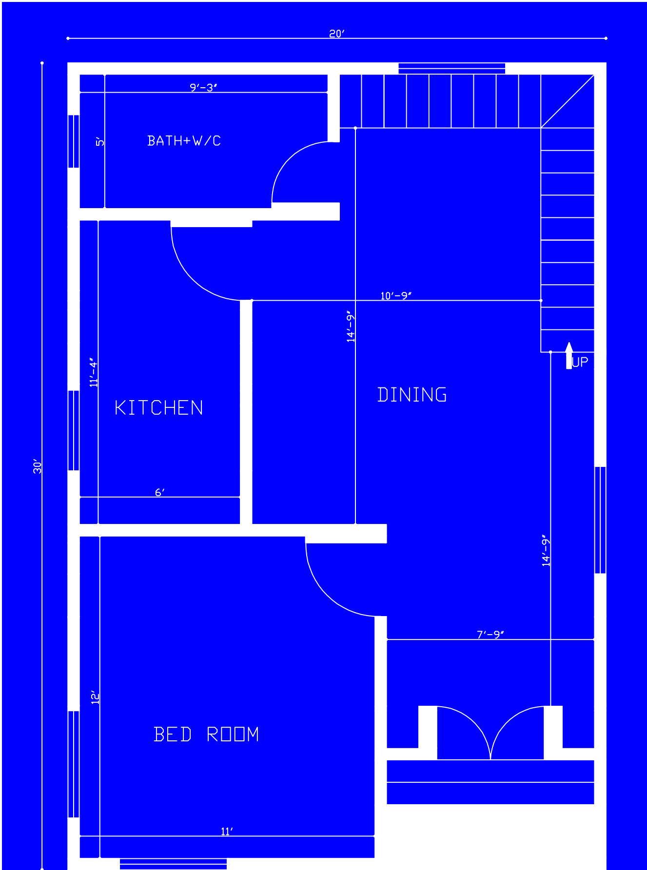
30'x20' 1 Bedroom House Plan
