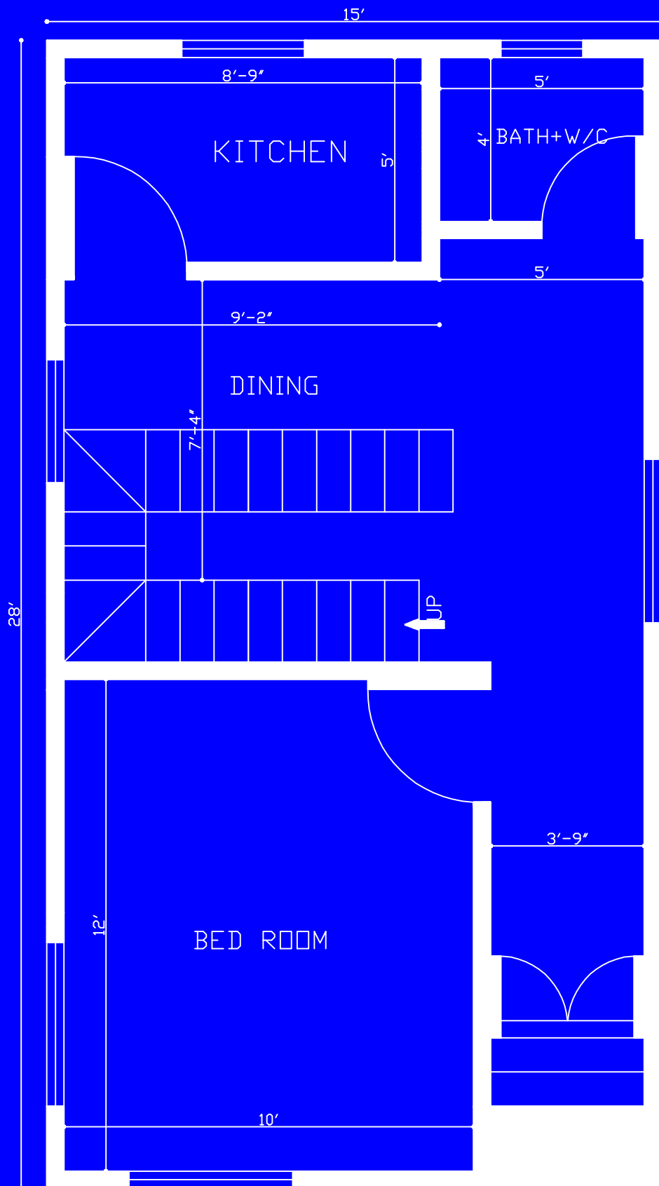
28'x15' 1 Bedroom House Plan
