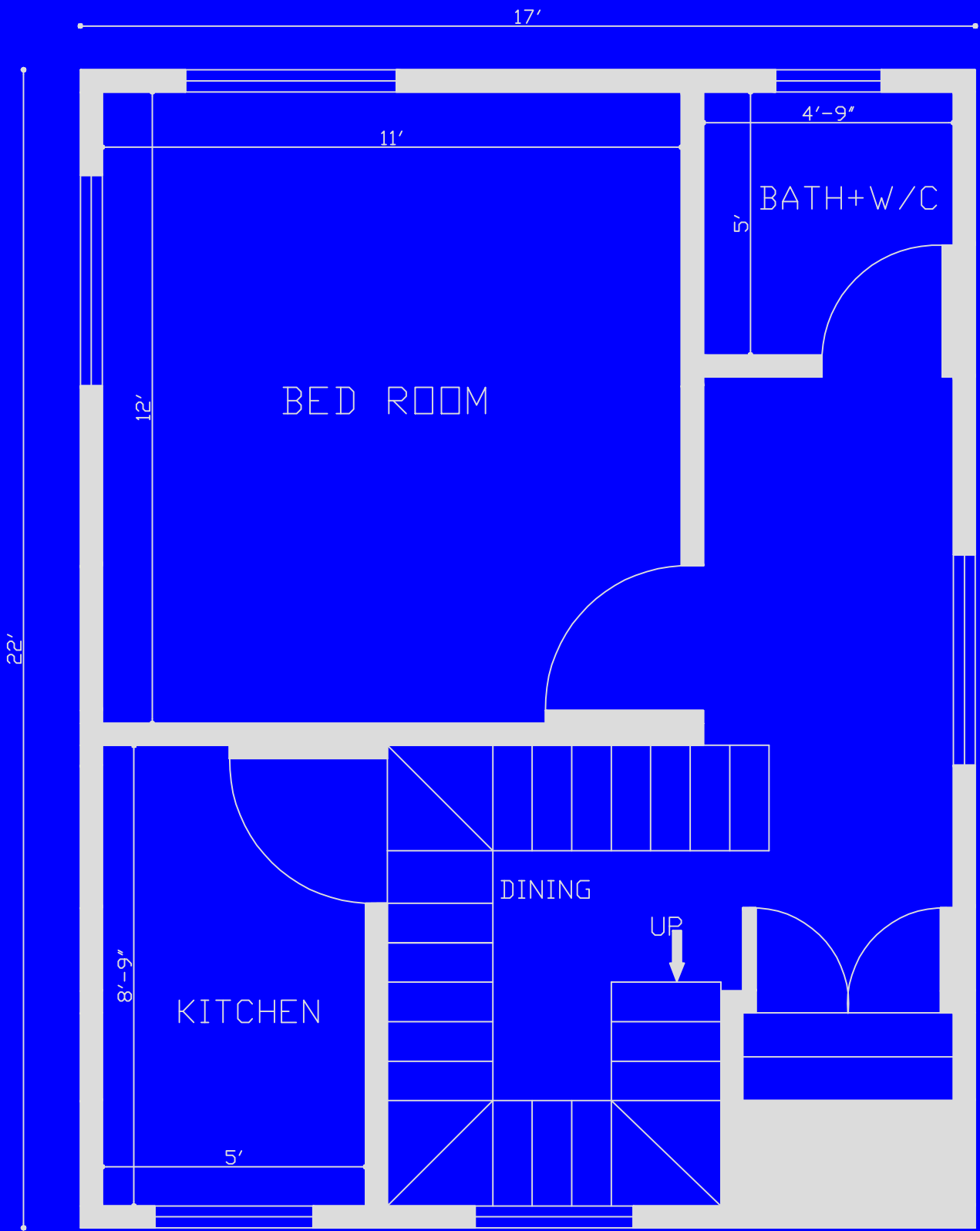
22'X17' 1 Bedroom House Plan
