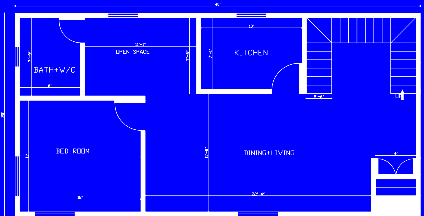
20'x40' 1 Bedroom House Plan
