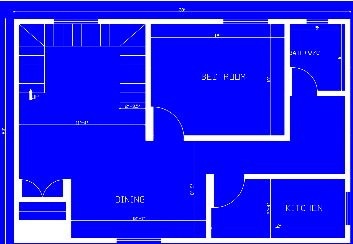
20'x30' 1 Bedroom House Plan
