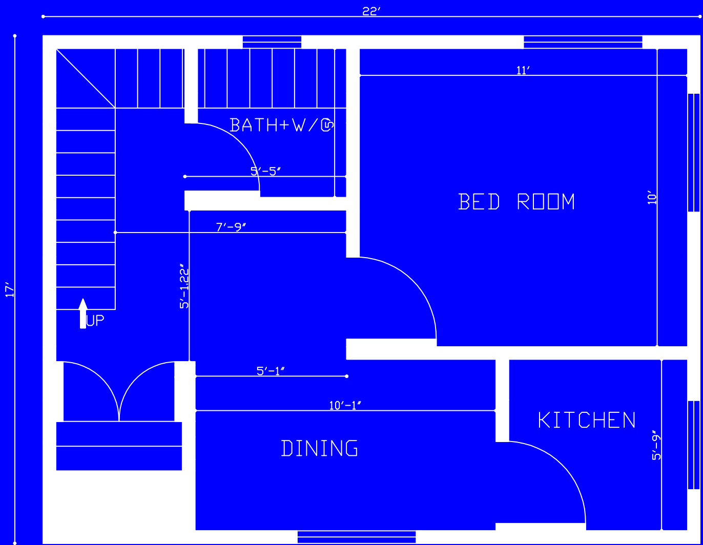
17'x22' 1 Bedroom House Plan
