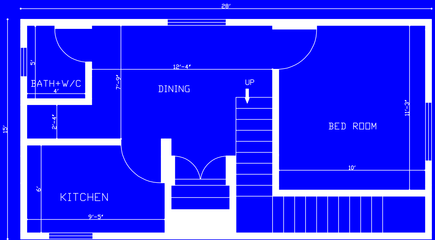
15'x28' 1 Bedroom House Plan
