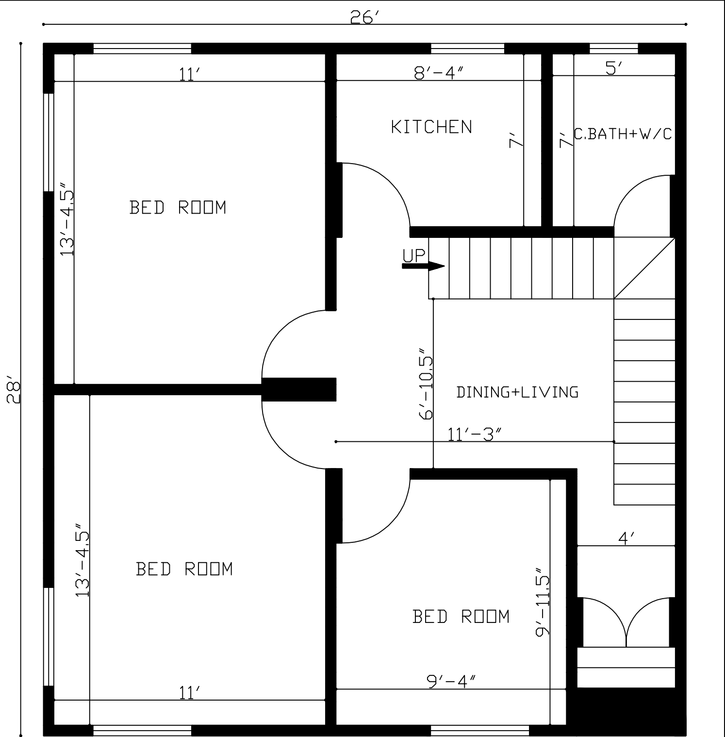
28'X26' 3Bhk House Plan
