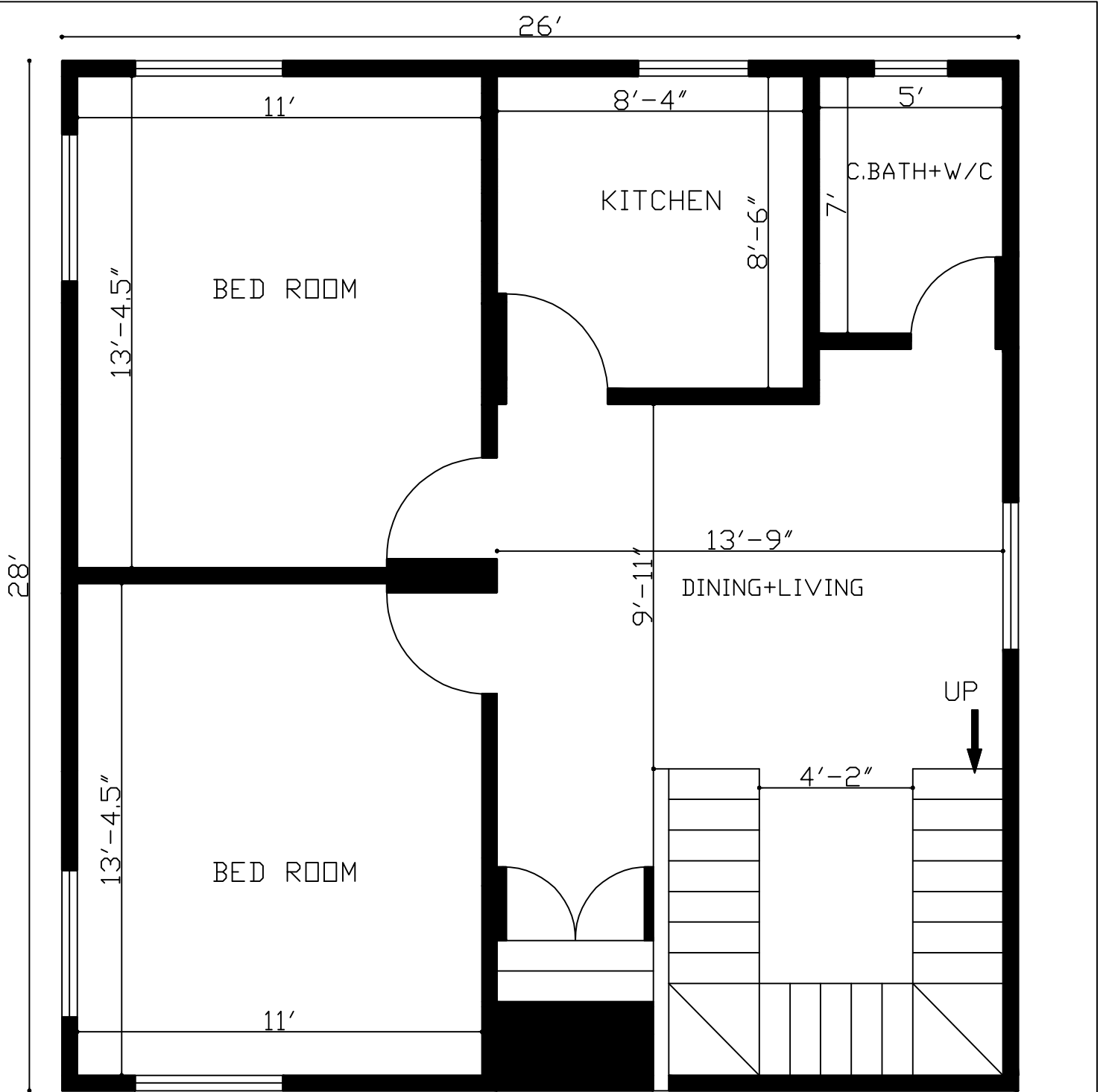
28'X26' 2Bhk House Plan
