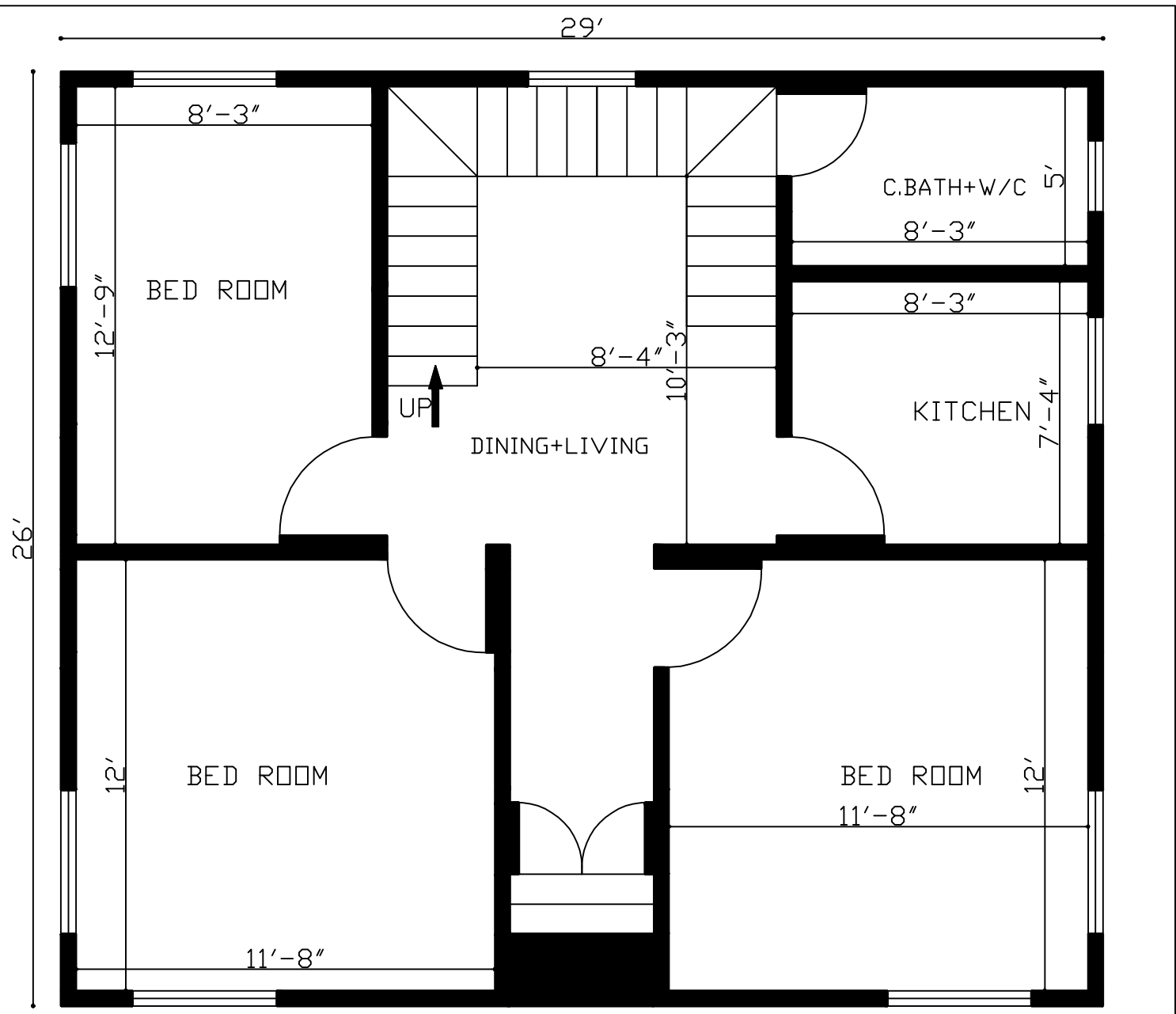
26'X29' 3Bhk House Plan
