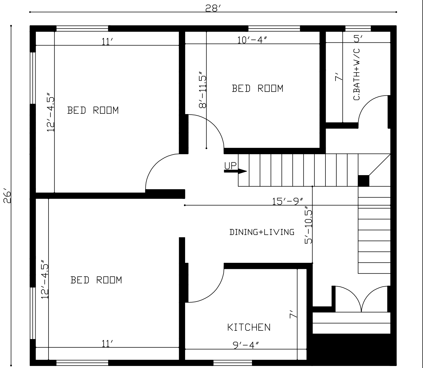
26'X28' 3Bhk House Plan
