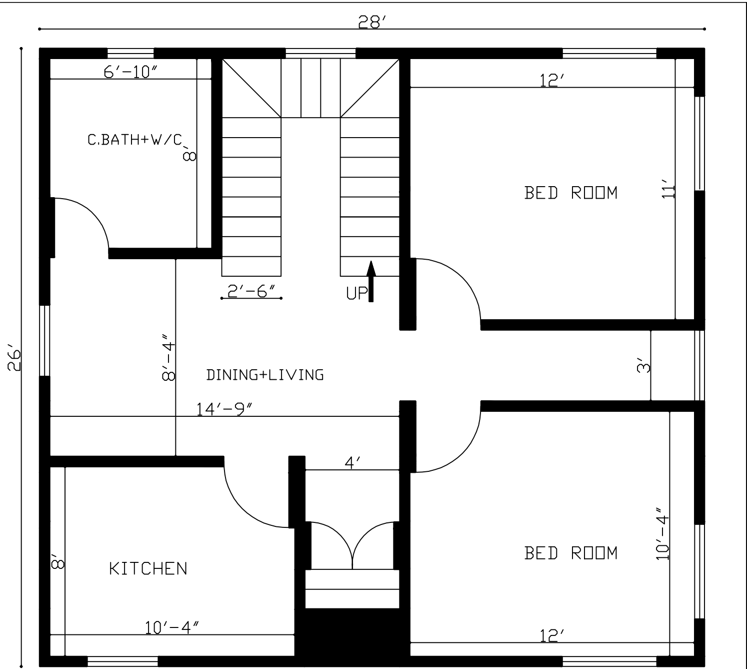
26'X28' 2Bhk House Plan
