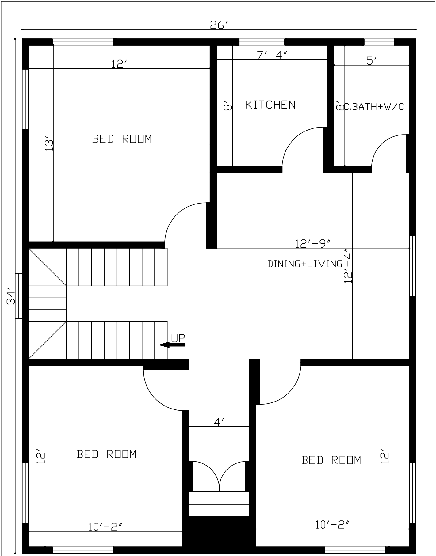
34'X26' 3Bhk House Plan
