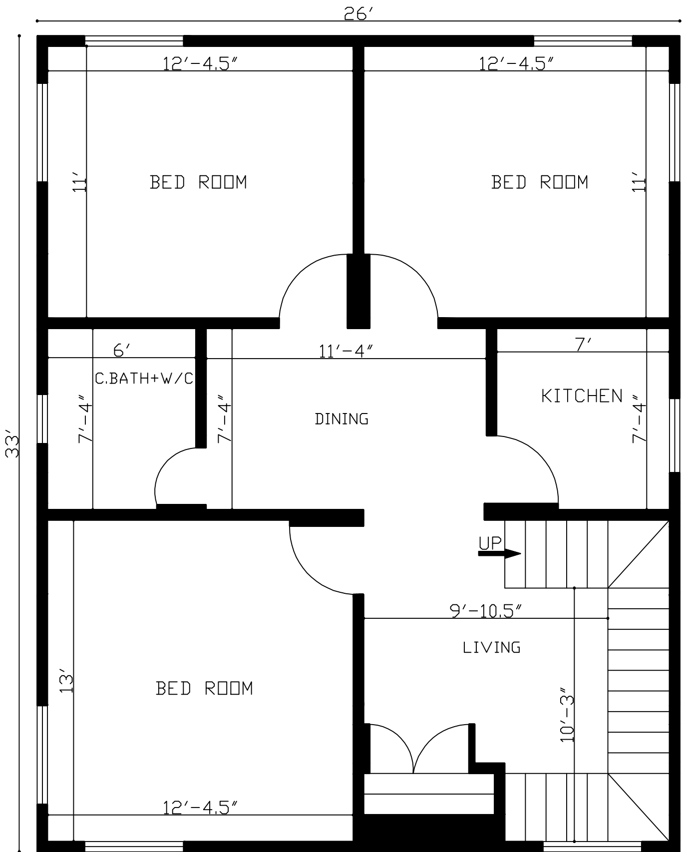
33'X26' 3Bhk House Plan
