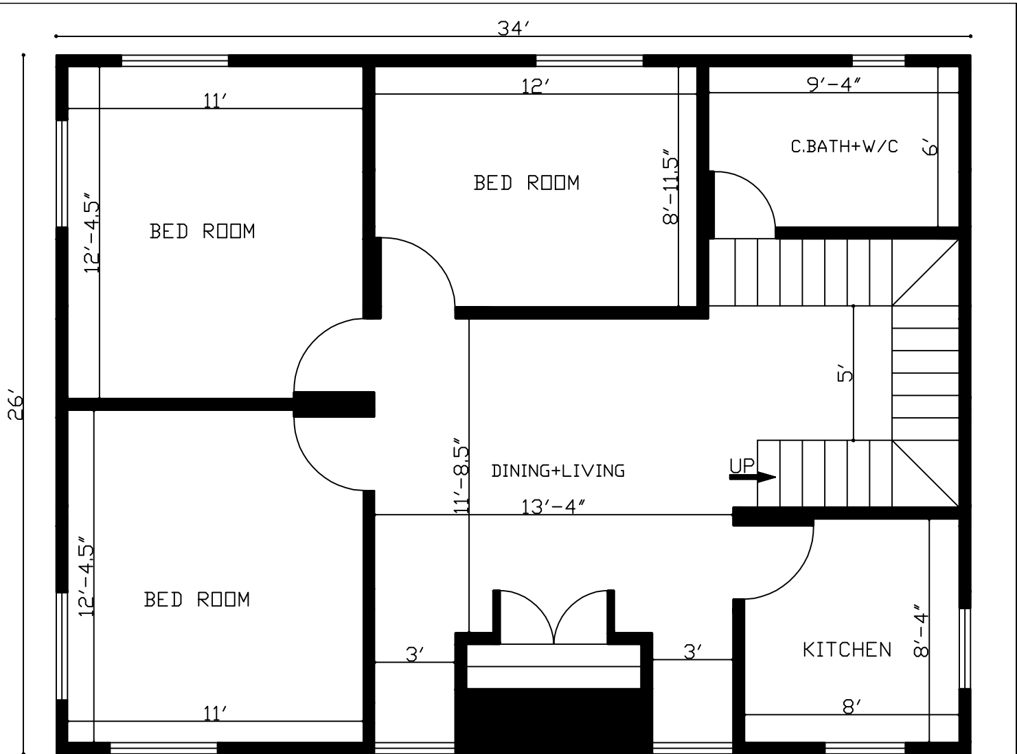
26'X34' 3Bhk House Plan
