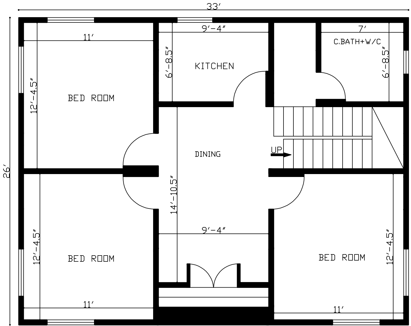
26'X33' 3Bhk House Plan
