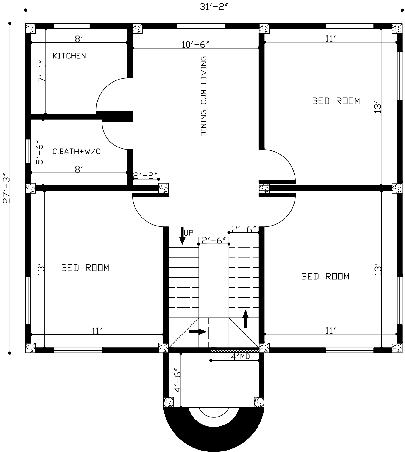
31' X 27' 3 BHK HOUSE PLAN
