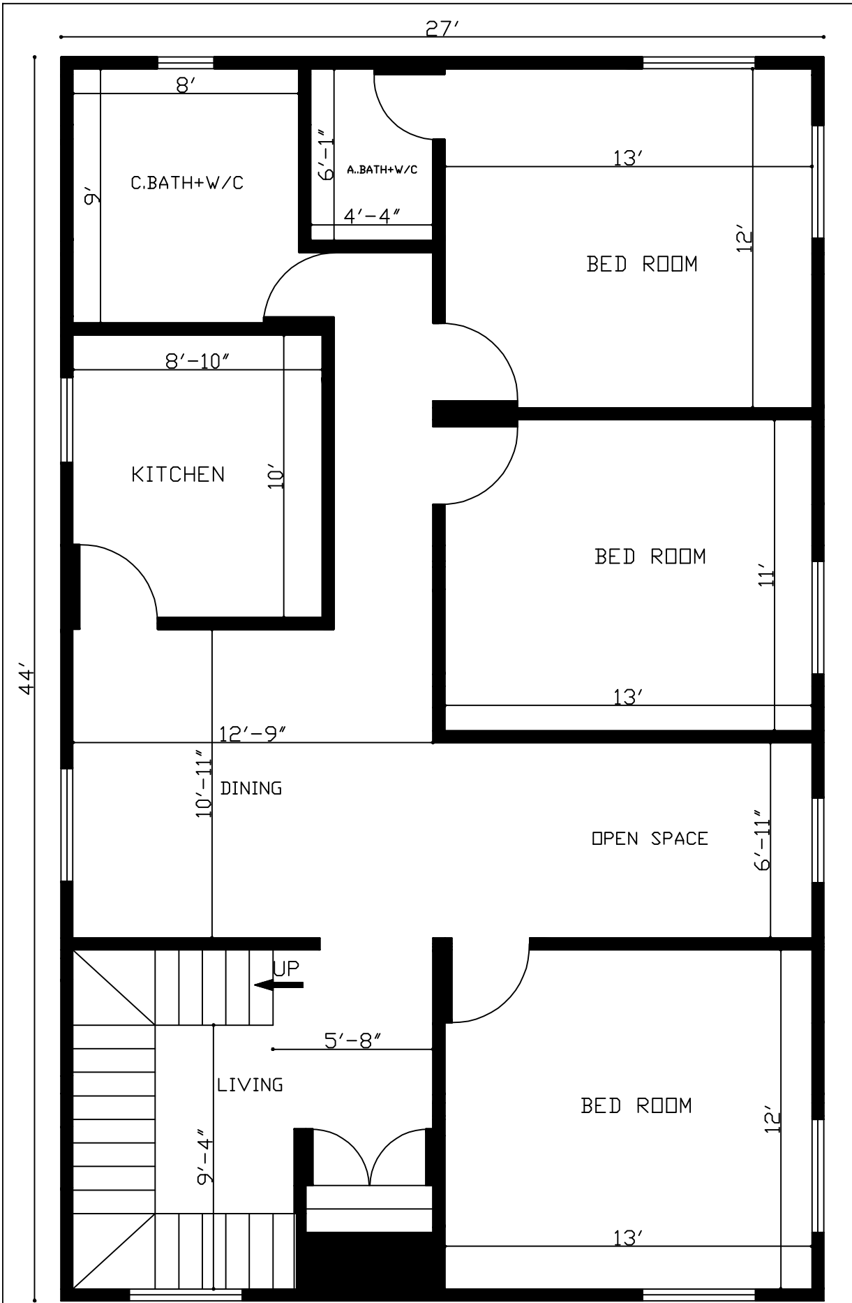
44'X27' 3Bhk House Plan
