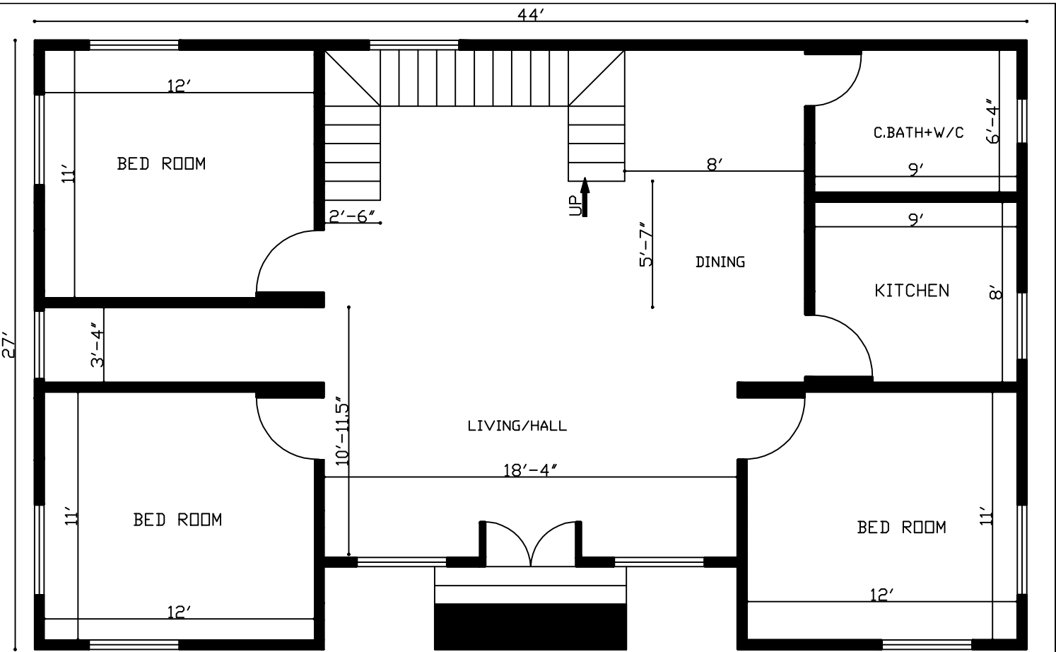
27'X44' 3Bhk House Plan
