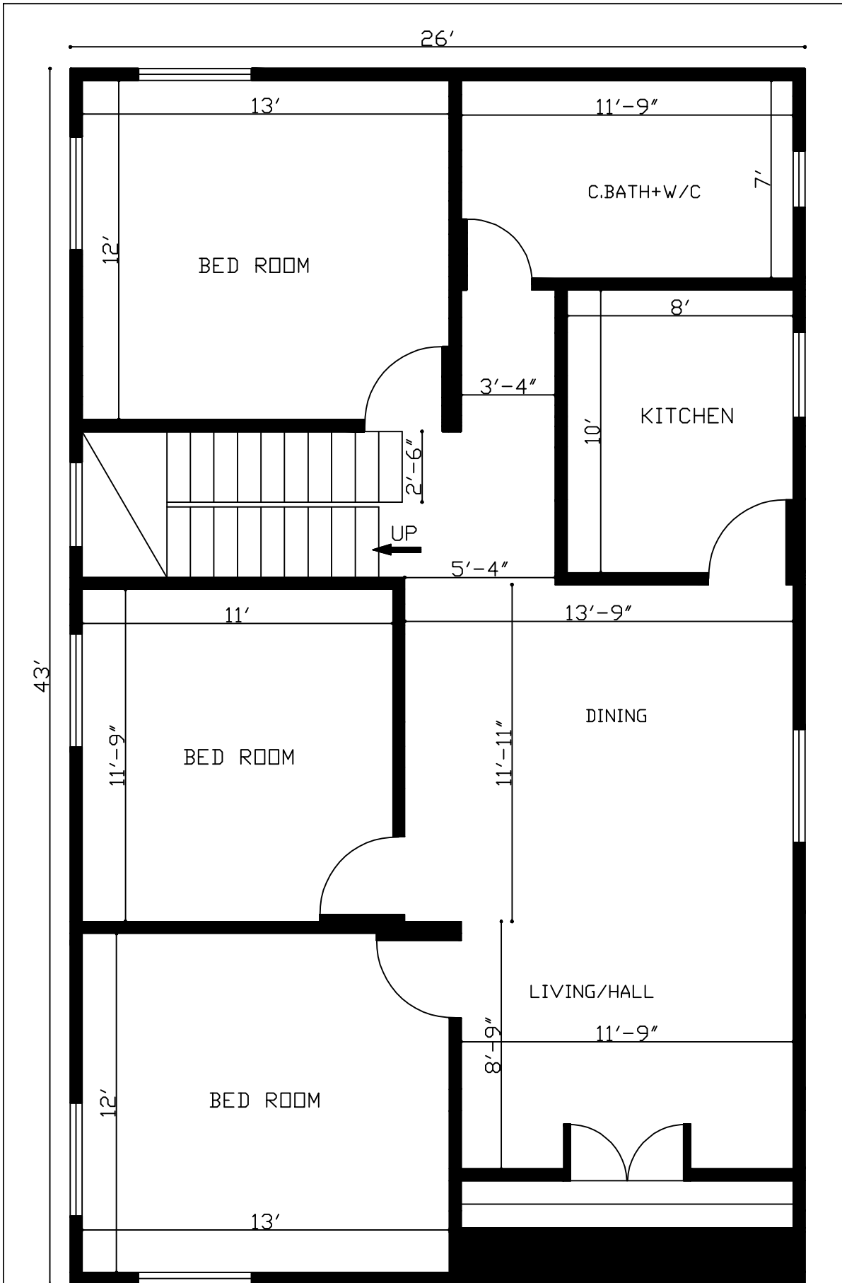
43'X26' 3Bhk House Plan
