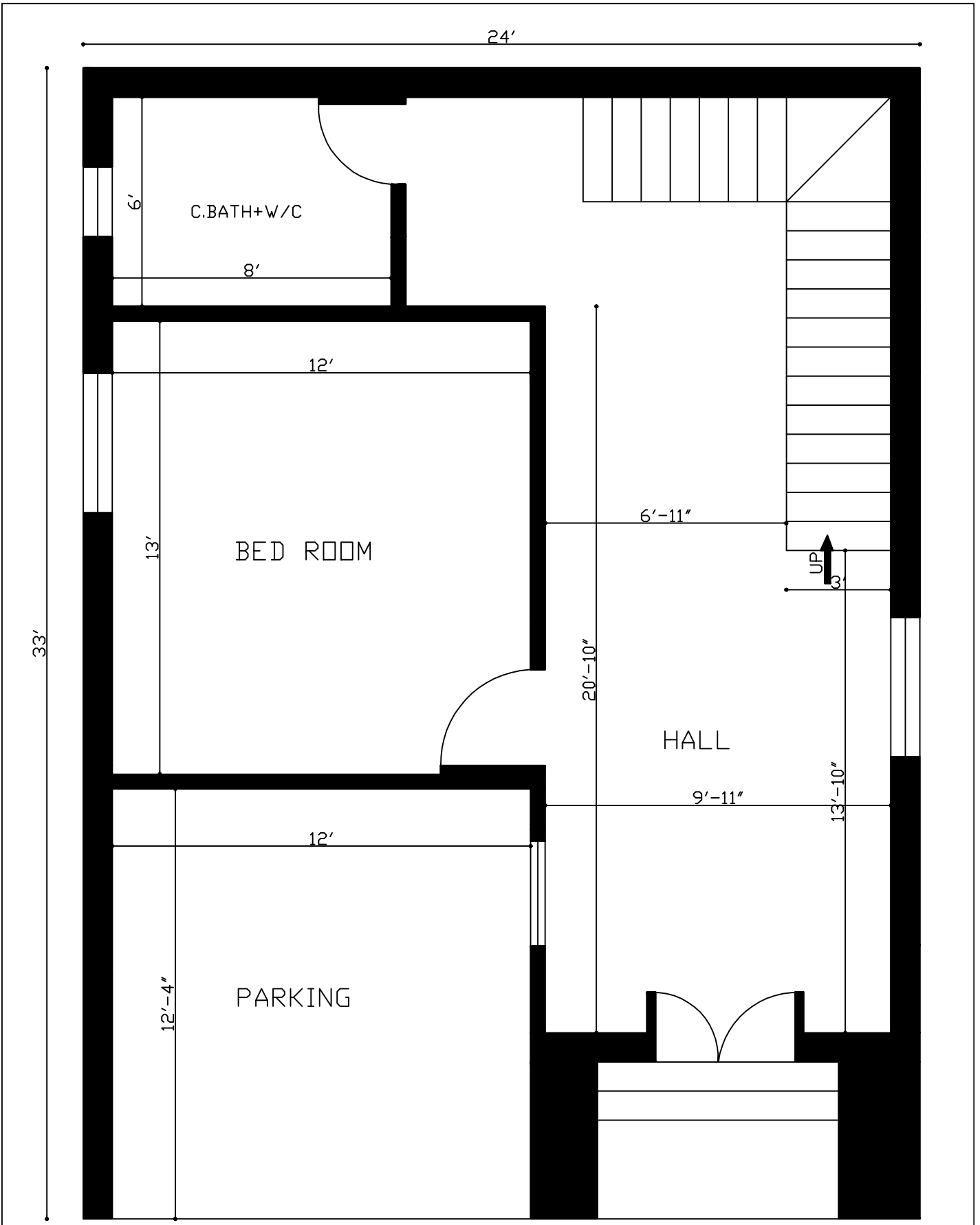
33'x24' Duplex House Plan (Ground Floor)
