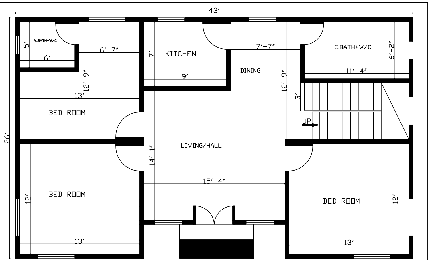
26'X43' 3Bhk House Plan
