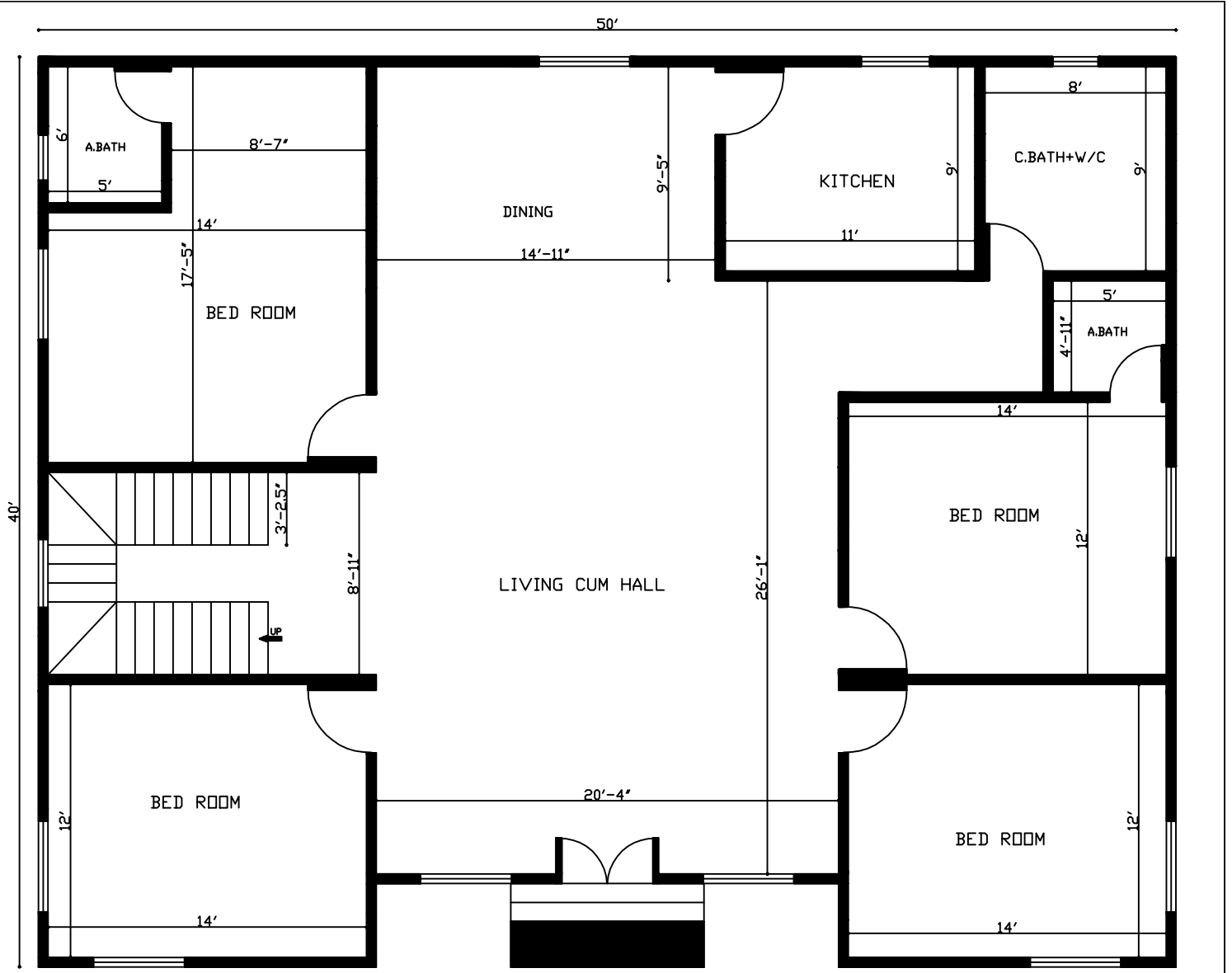
4 Bhk House Plan In 2000 Sq. Ft. (40'x50')
