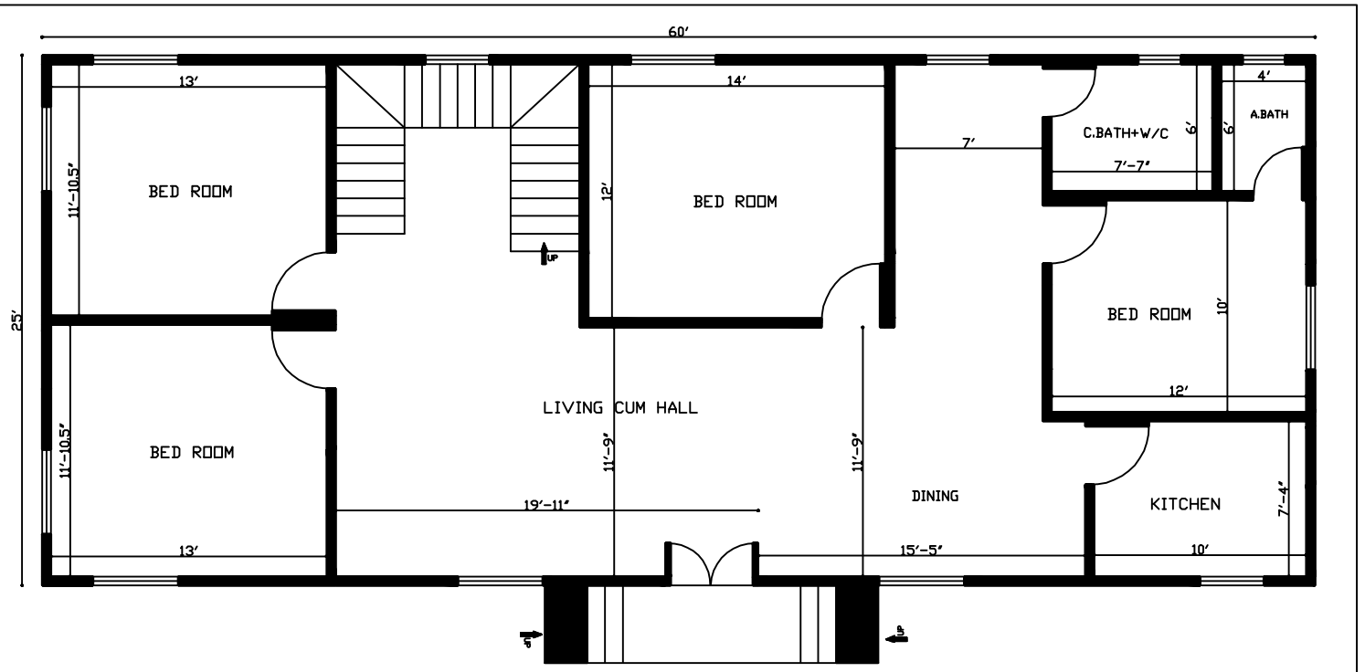
4 Bhk House Plan In 1500 Sq. Ft. (60'x25')
