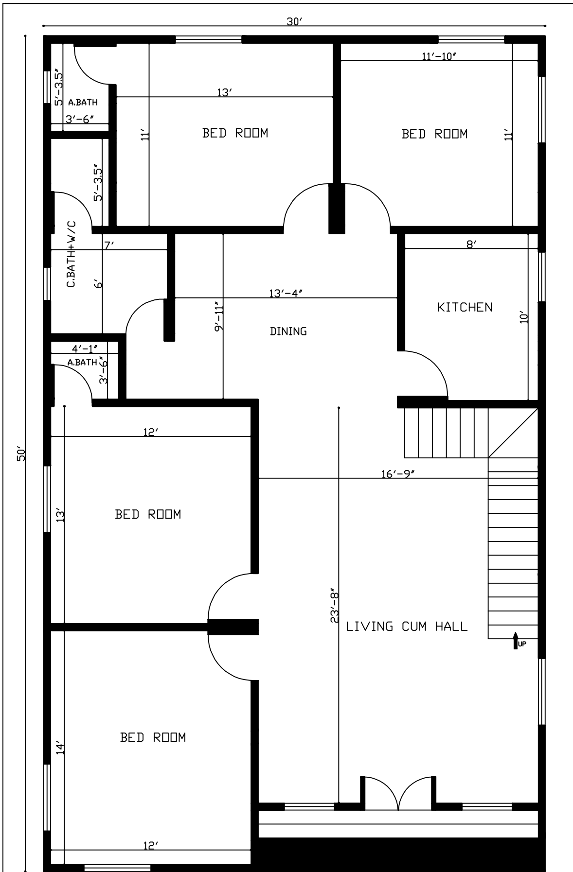
4 Bhk House Plan In 1500 Sq. Ft. (50'x30')
