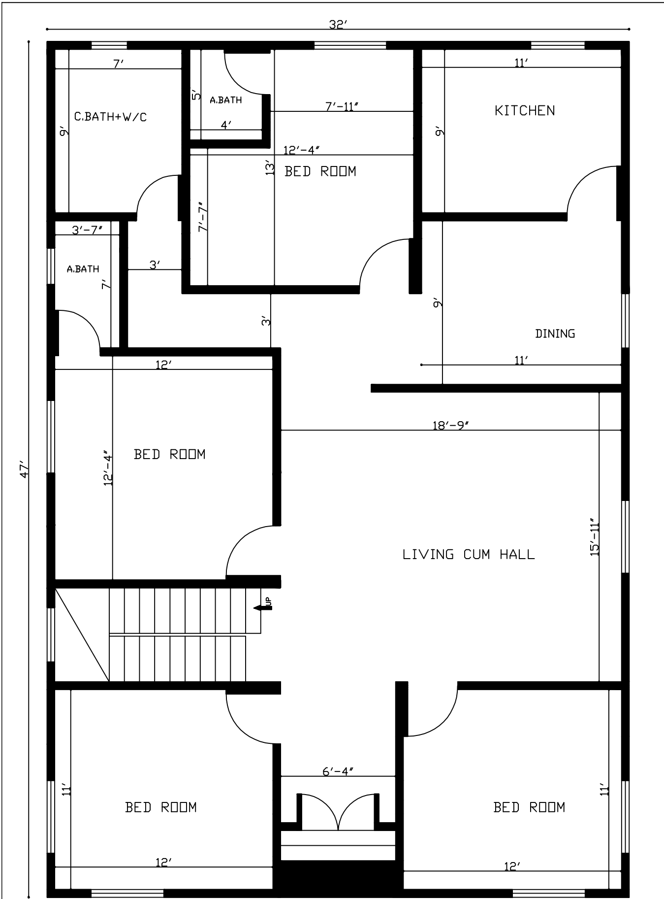
4 Bhk House Plan In 1500 Sq. Ft. (47'x32')
