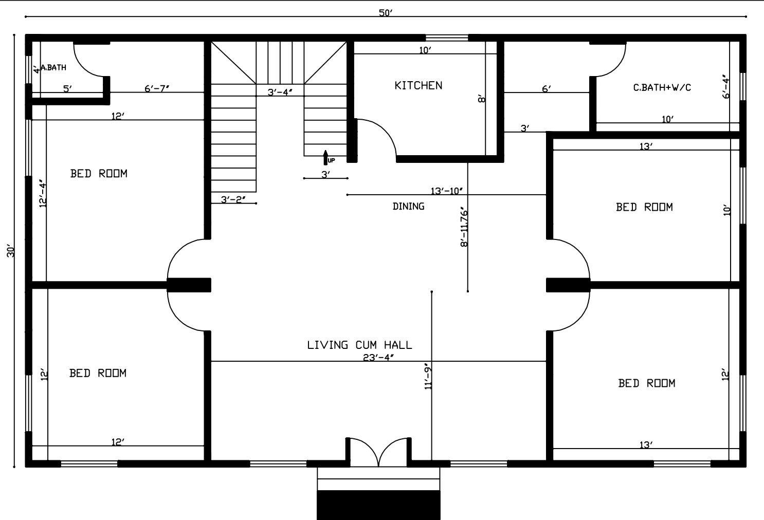
4 Bhk House Plan In 1500 Sq. Ft. (30'x50')
