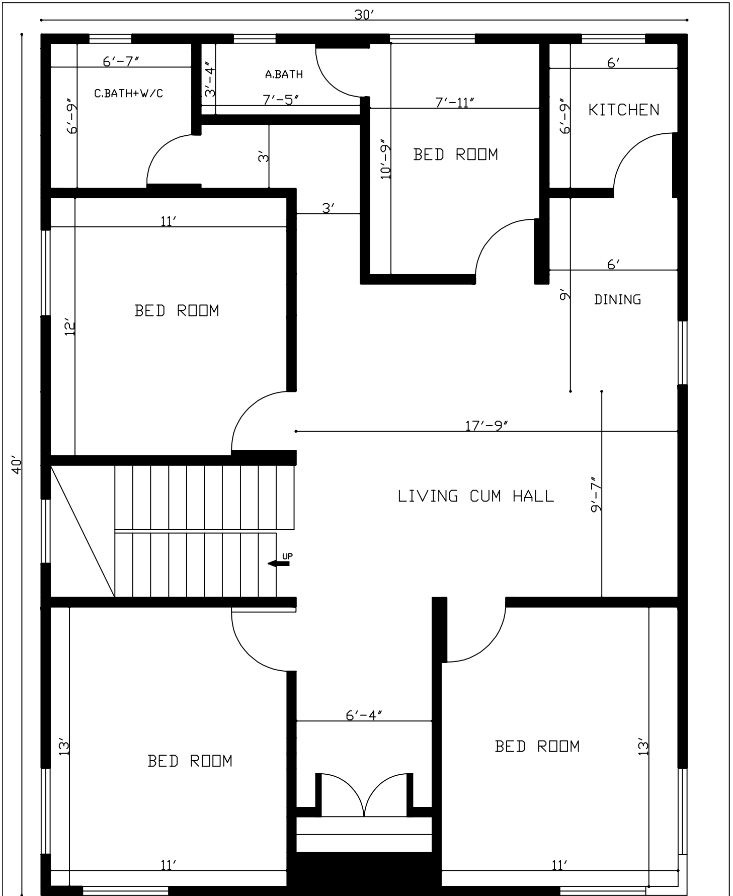
4 Bhk House Plan In 1200 Sq. Ft. (40'x30')
