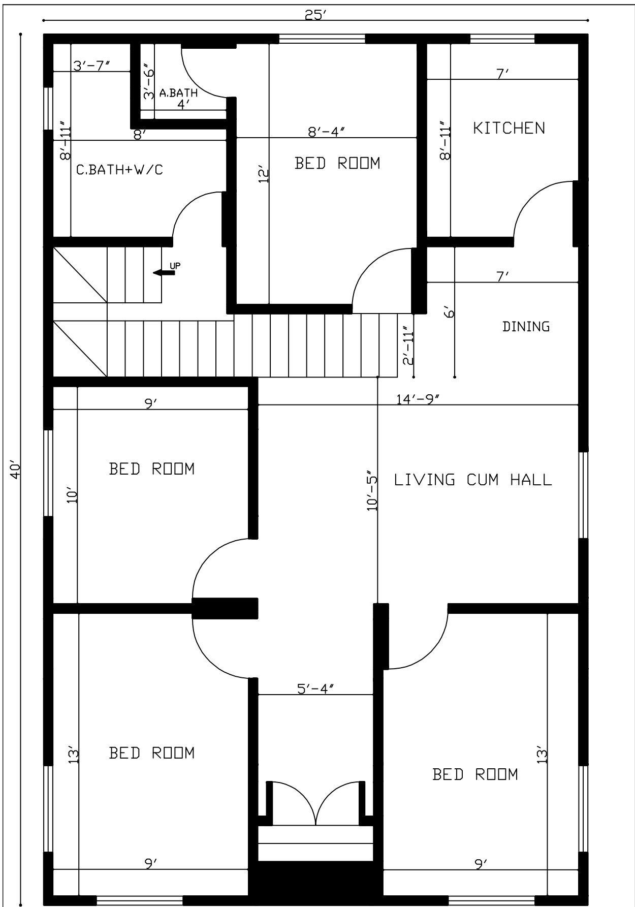
4 Bhk House Plan In 1000 Sq. Ft. (40'x25')
