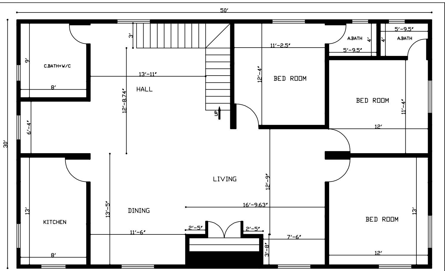
3bhk House Plan In 1500 Sq. Ft.
