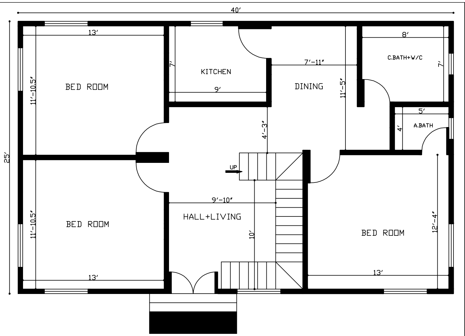
3bhk House Plan In 1000 Sq. Ft.
