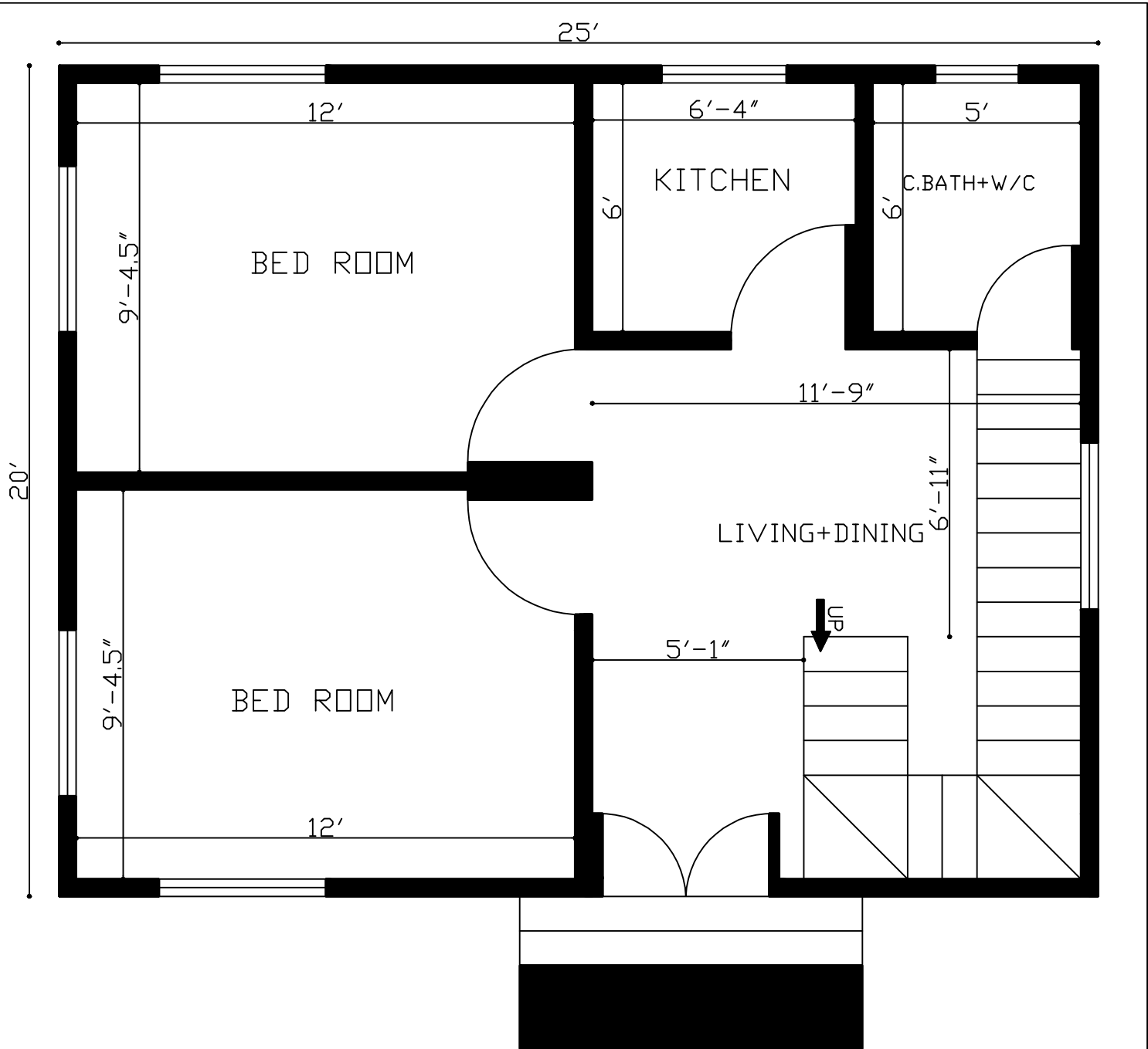
2 Bhk House Plan In 500 Sq. Ft.
