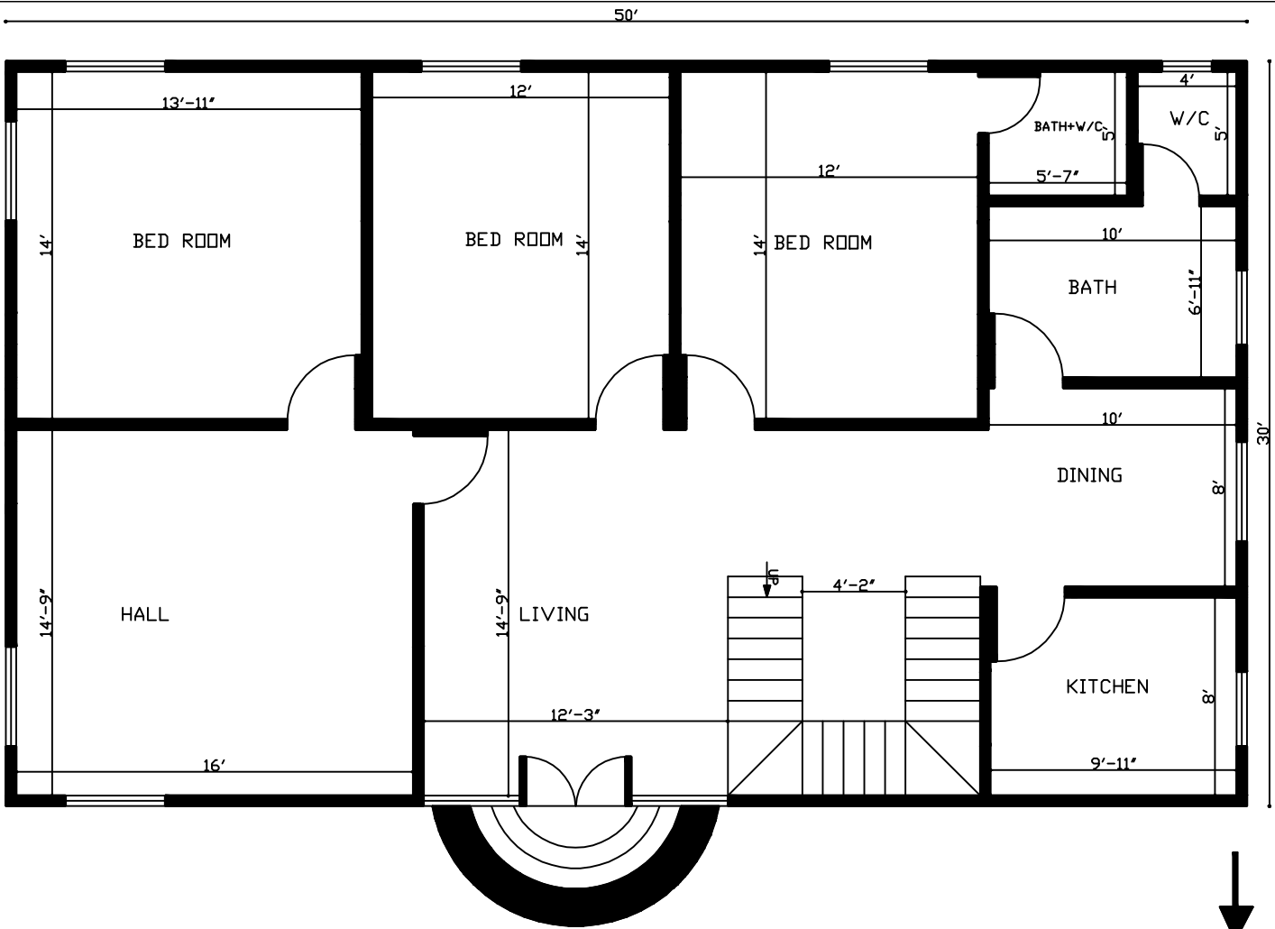
50'x30' 3 Bhk East Facing House Plan
