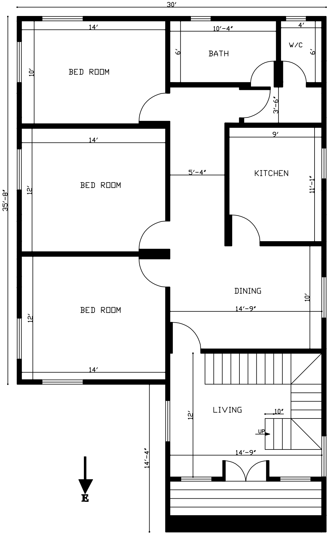
50'x30' 3 Bedroom East Facing House Plan
