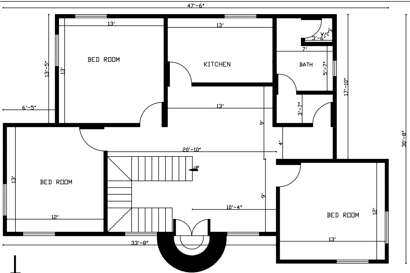
48'X31' 3 Bedroom South Facing House Plan
