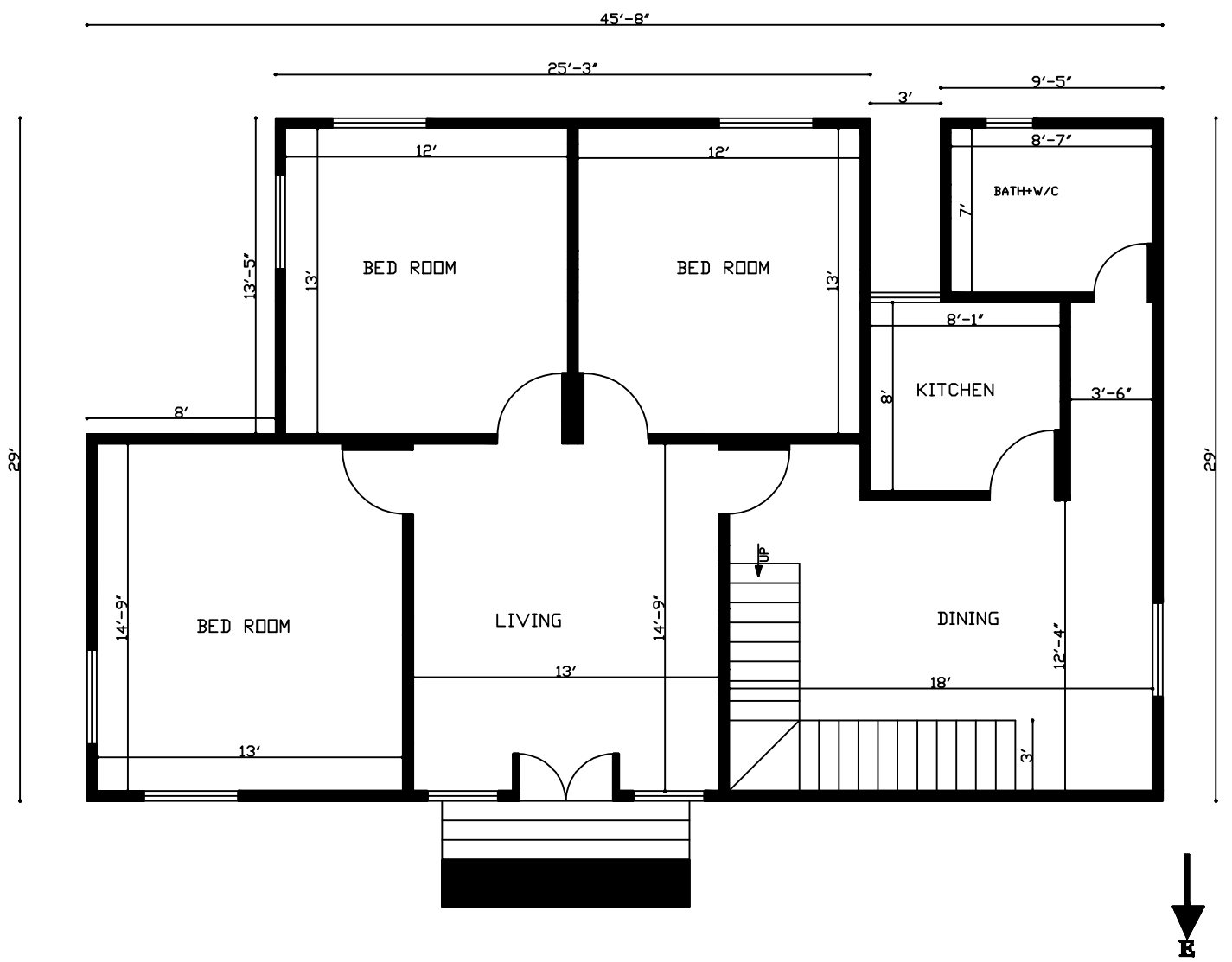
46'x29' 3 Bedroom East Facing House Plan
