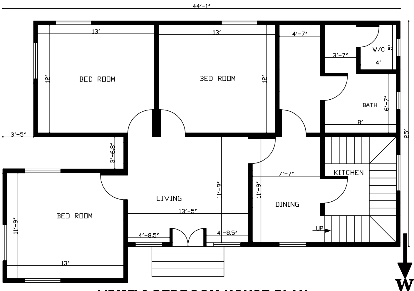
44'X25' 3 BEDROOM HOUSE PLAN
