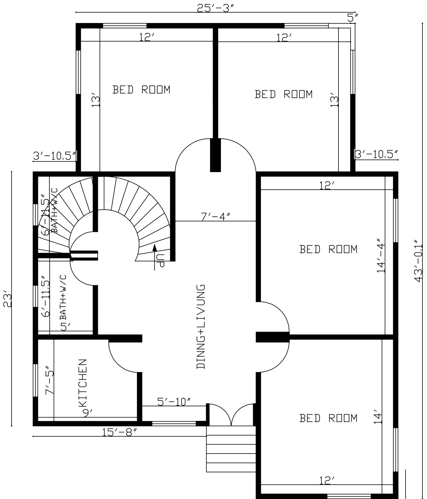
43'x28' 4 BEDROOM HOUSE
