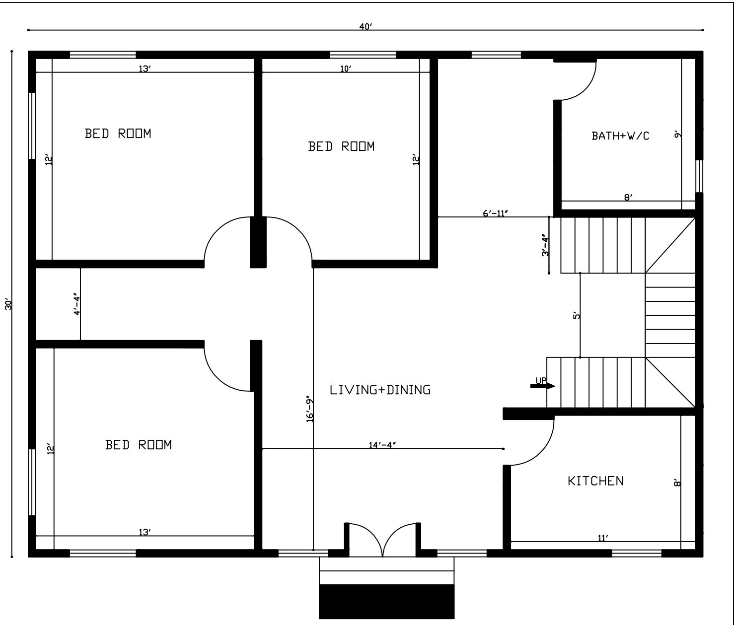
40'x30' 1200 Sq. Ft. House Plan
