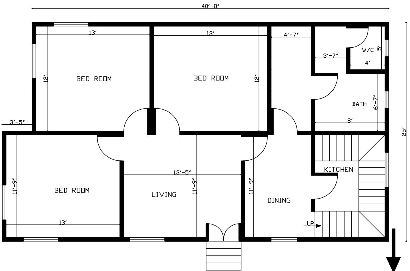
40'X25' 3 BEDROOM HOUSE PLAN
