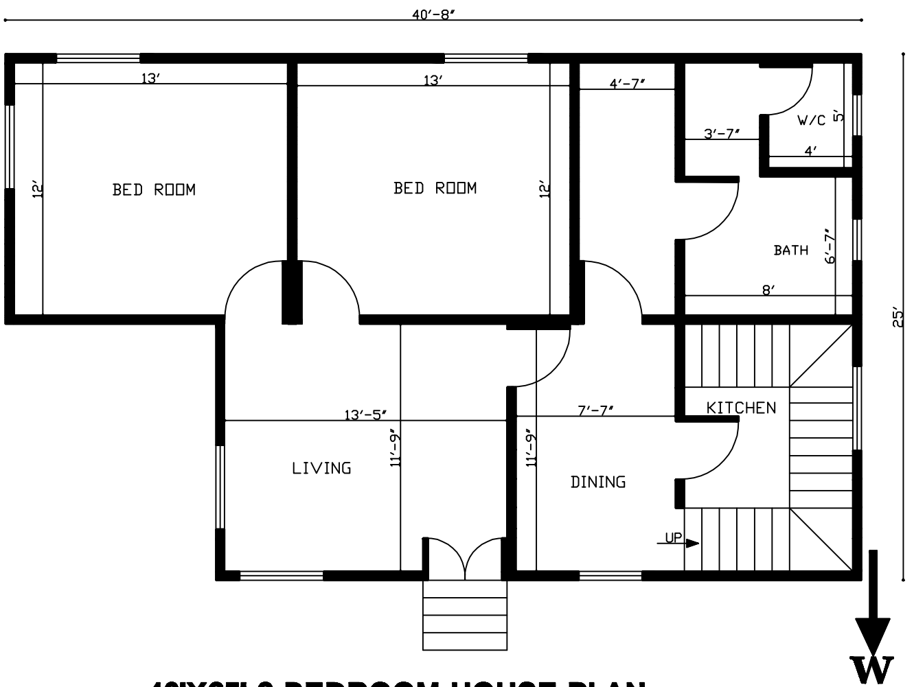
40'X25' 2 BEDROOM HOUSE PLAN
