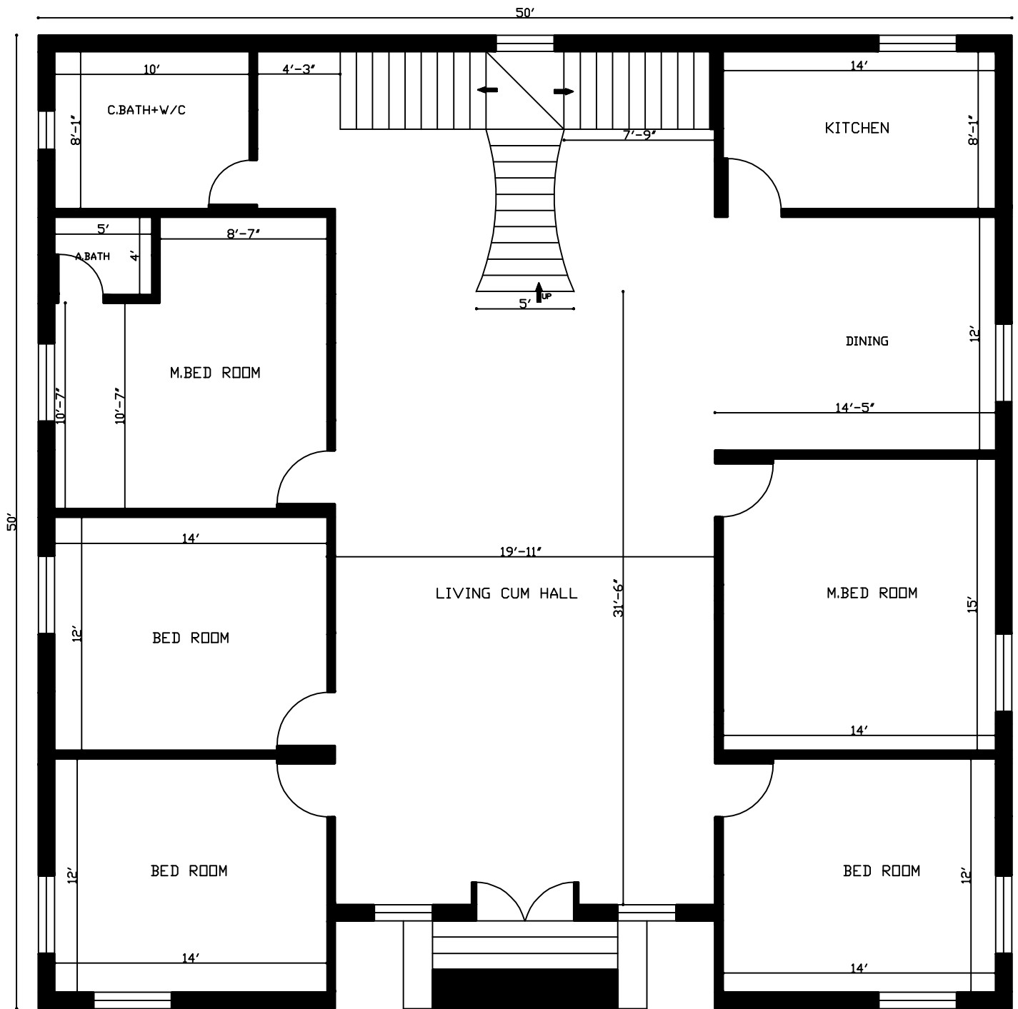
4 Bhk House Plan In 2500 Sq. Ft.
