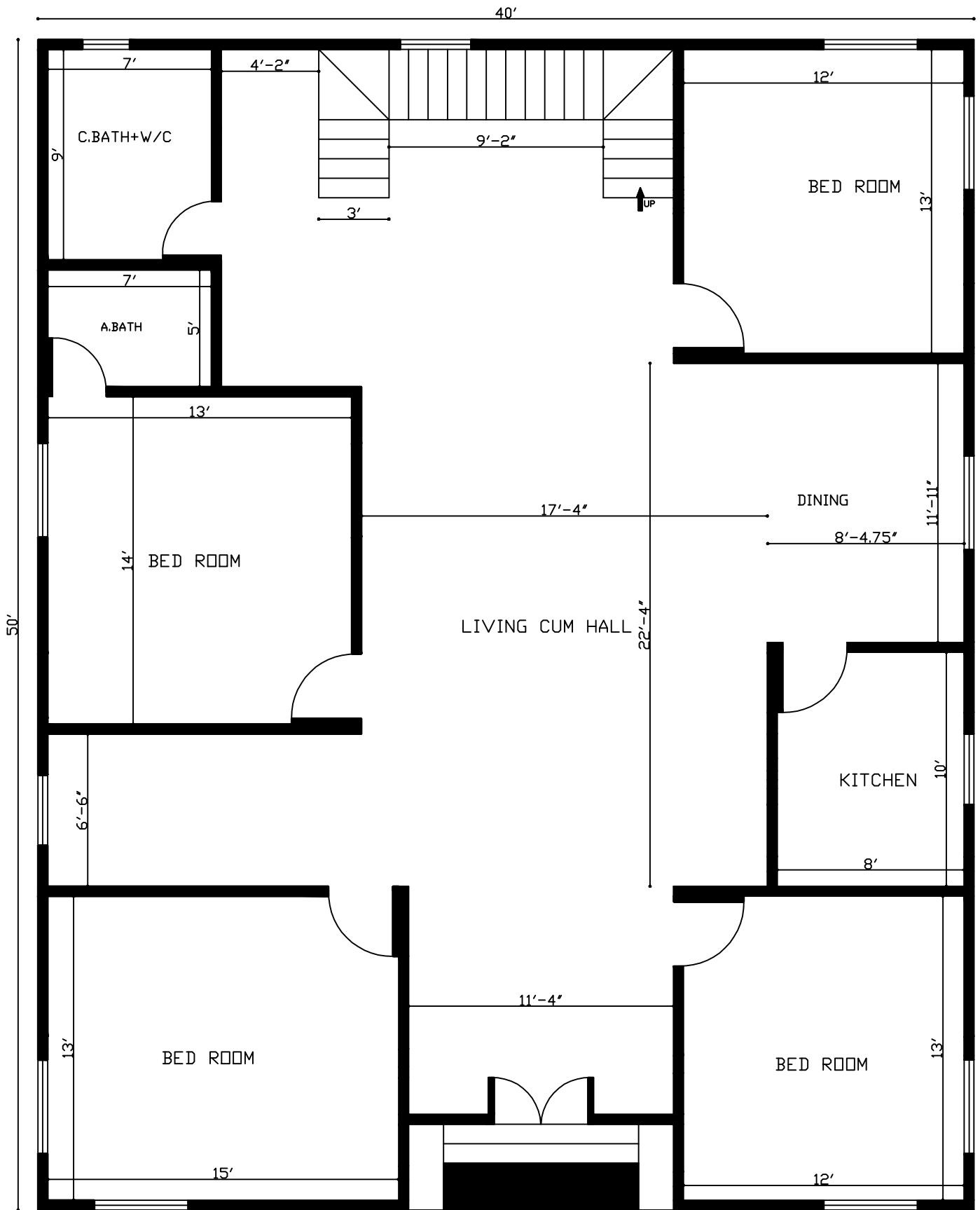
4 Bhk House Plan In 2000 Sq. Ft.
