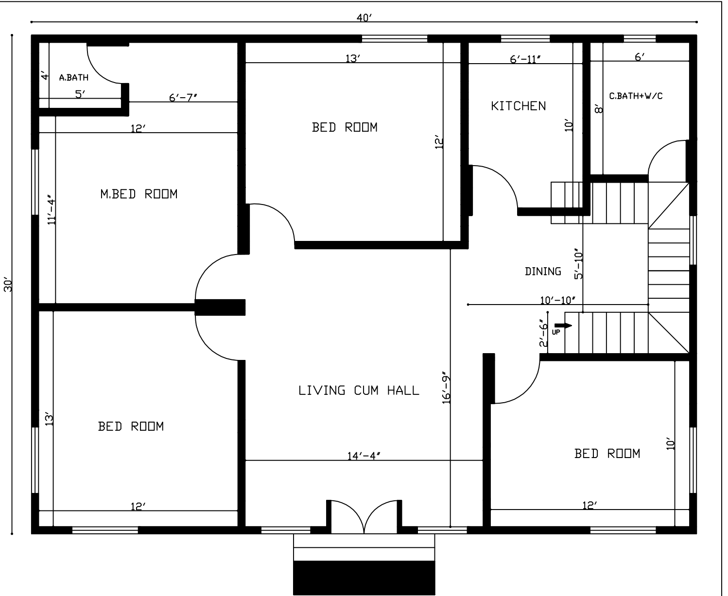
4 Bhk House Plan In 1200 Sq. Ft.
