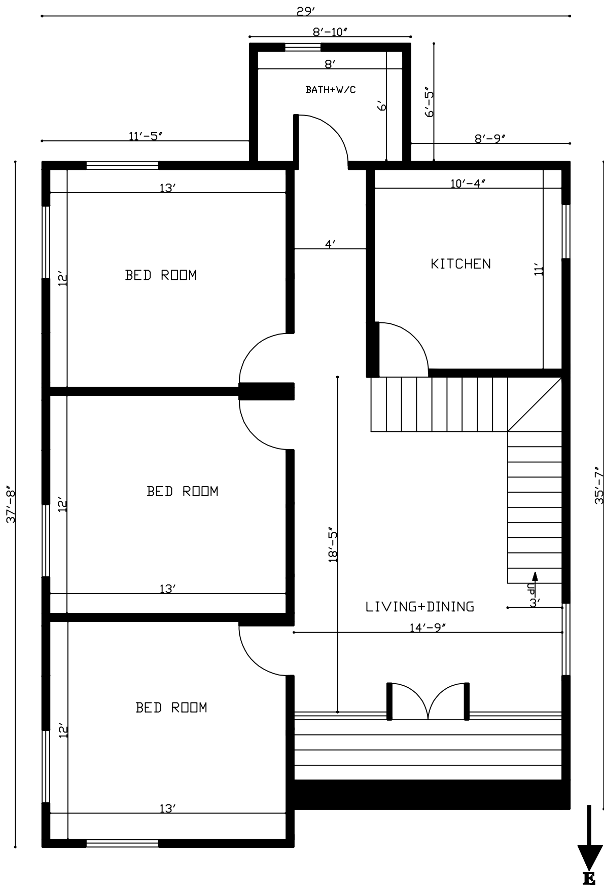
38'x29' 3 Bedroom East Facing House Plan
