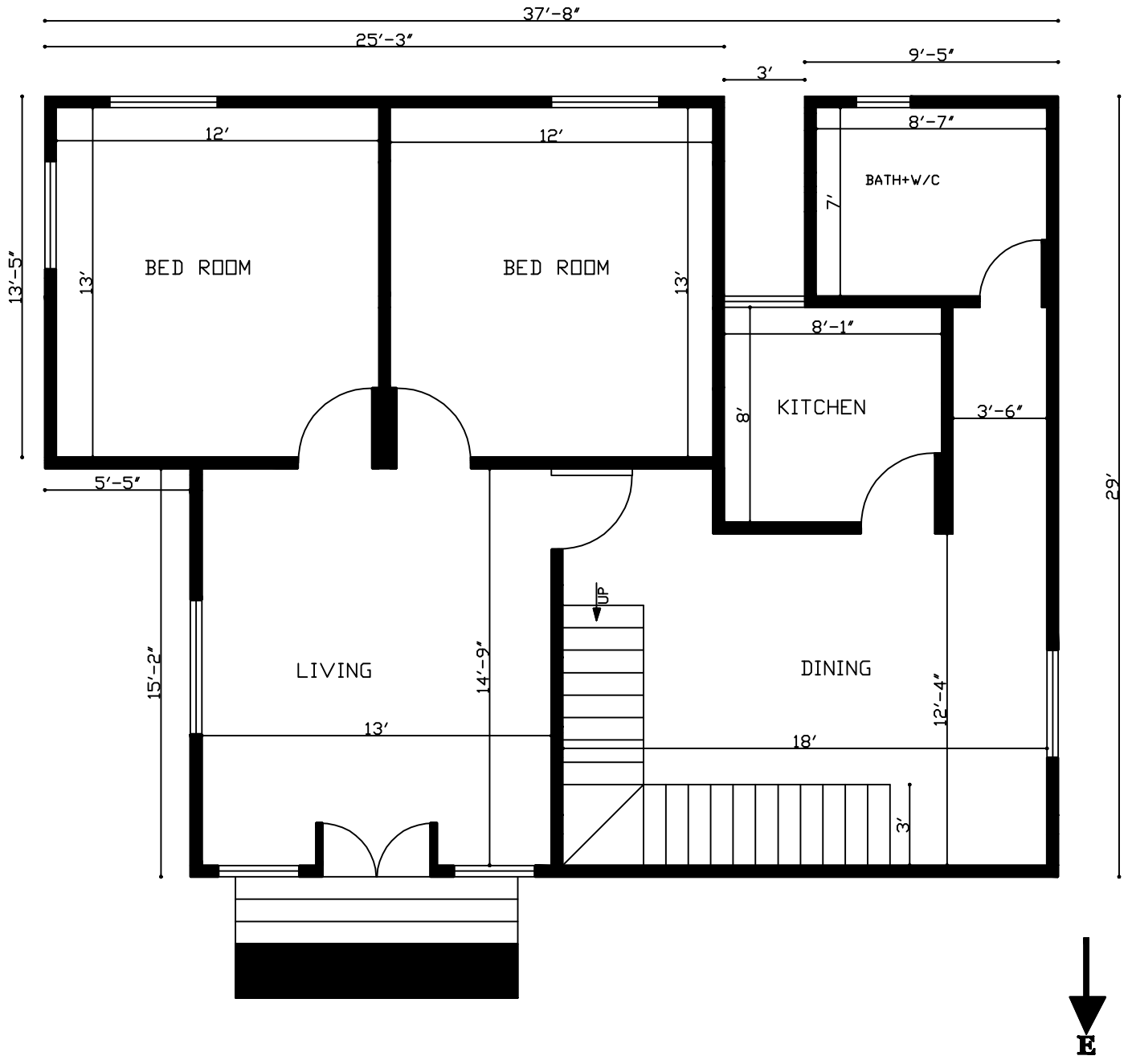
38'x29' 2 Bedroom East Facing House Plan
