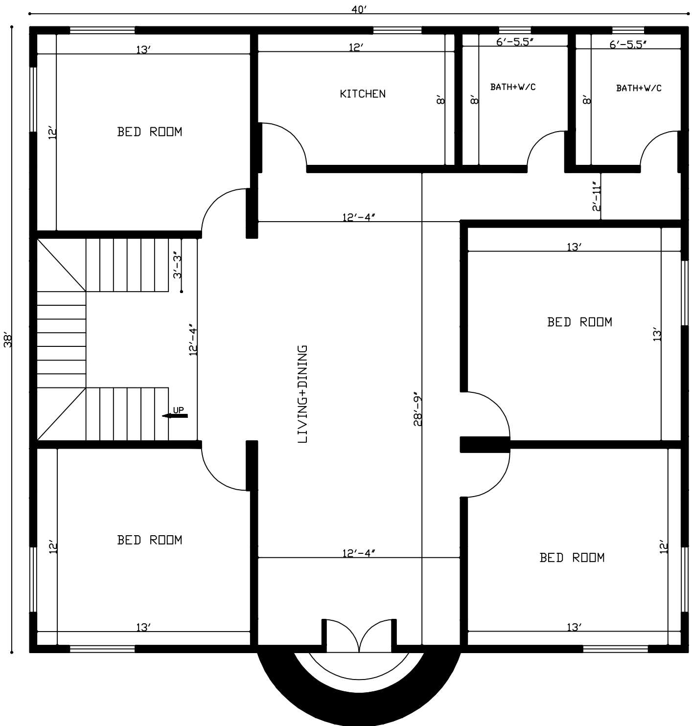
38'X40' 1500 Sq. Ft. House Plan
