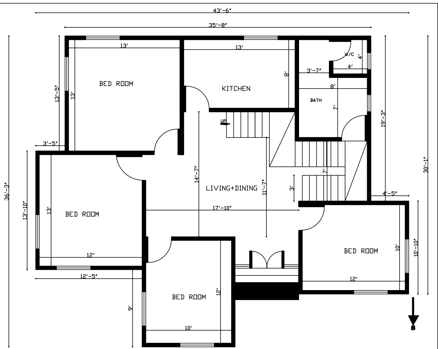
36'X44' 4 Bedroom South Facing House Plan
