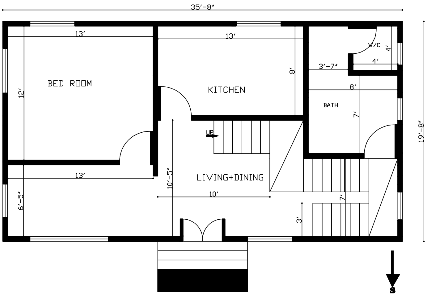
36'X20' 1 Bedroom South Facing House Plan
