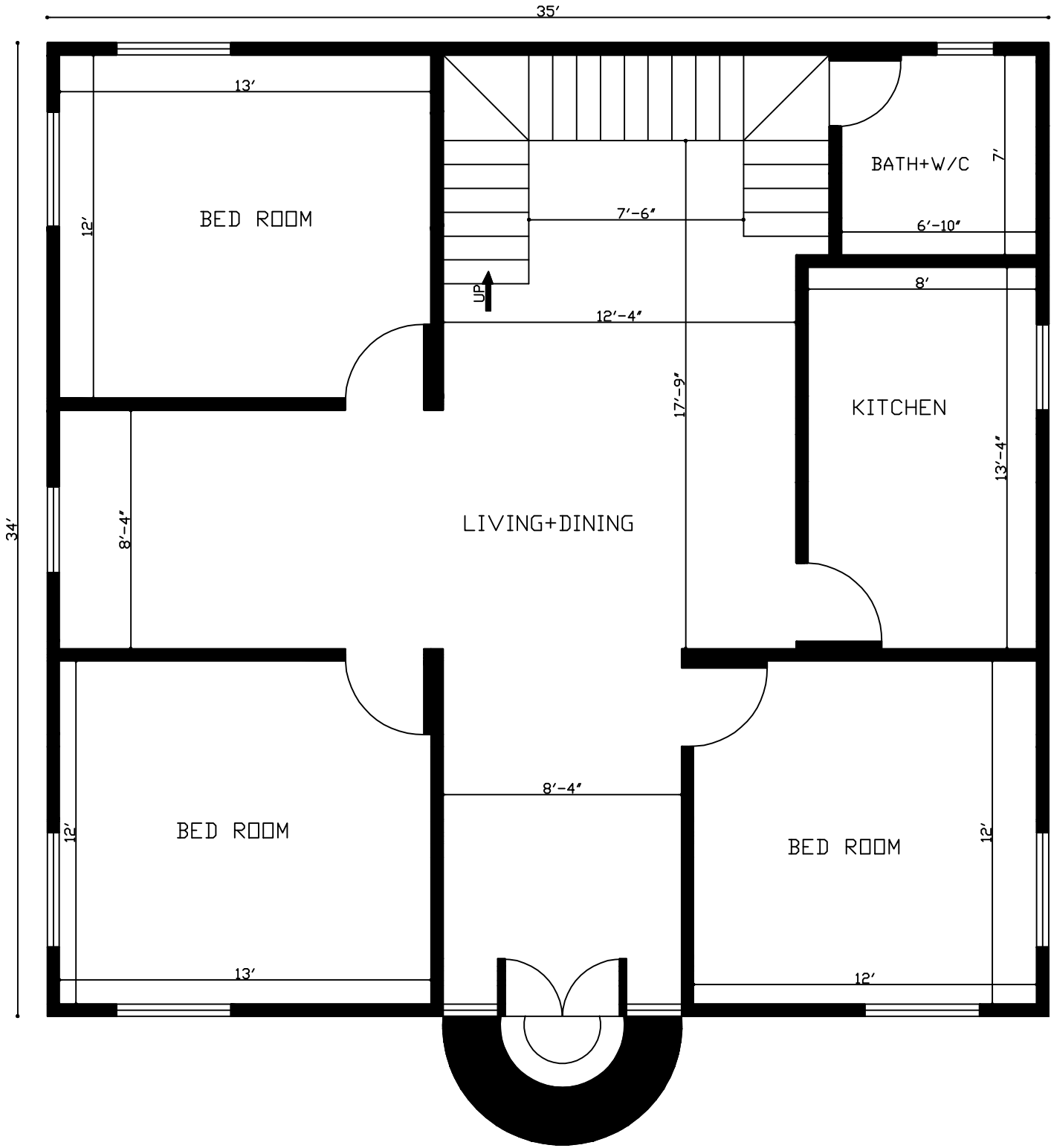
34'x35' 1200 Sq. Ft. House Plan
